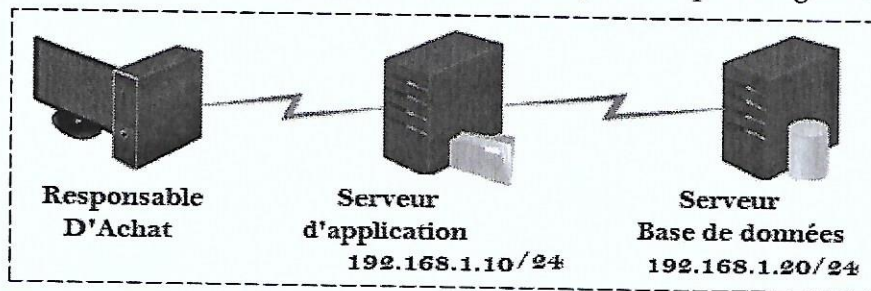
Figure 4 : Architecture client/serveur
